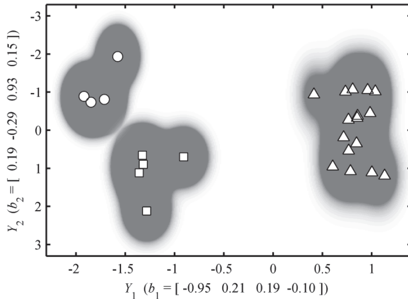
Figure 46. Class-conditional probability densities are shown for a discriminant subspace composed of the four most salient empirical features ( R_{35} , F6 , E6 , and A' ). Class probabilities are indicated by shading from gray (100%) through white (probabilities approach zero or equal values for two or more classes). Observations of Full Charge ( \circ ), Charge 1 ( \square ), and Charge 2 ( \Delta ) projected into the subspace have class separation \Lambda = 48.3 .
