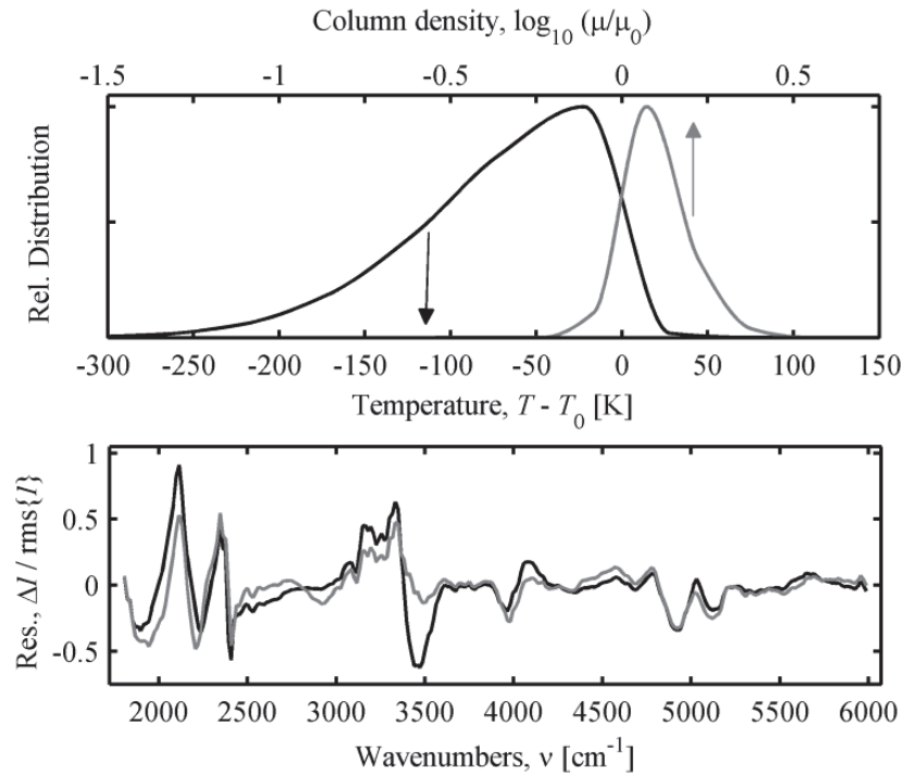
Figure 36. HE and distribution model fits to a combusting plume. Upper panel: distributions of temperature (—) and H 2 O column density (---) centered at T_0 = 1472 K and \mu_0 = \mu_{\text{H}_2\text{O}} = 4.7 \times 10^{20} \text{ cm}^{-2} . CO 2 and CO have the same column density distribution centered at \mu_{\text{CO}_2} = 1.6 \times 10^{21} \text{ cm}^{-2} and \mu_{\text{CO}} = 8.9 \times 10^{19} \text{ cm}^{-2} . Lower panel: Residuals between observed spectral intensity and distribution (—) and HE (---) models. RMS error is reduced from e = 21.5\% to e = 16.9\% when temperature and concentrations vary spatially.
