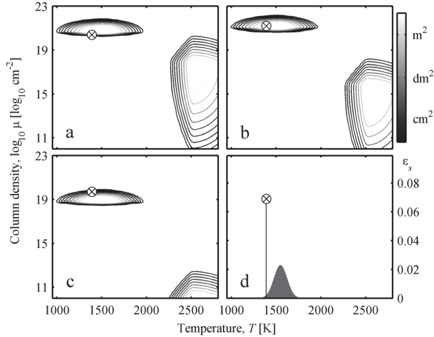
Figure 37. Distributions of a two-region model fit to the peak spectrum of a combusting muzzle plume. a) H 2 O, b) CO 2 , and c) CO compose an optically thick core of temperature near T \approx 1500 K and thin flame-front near T \approx 2550 K. Contours indicate relative area-weighting of emissions for the range of temperatures and concentrations. d) Soot emissivity distribution shows that most Planckian-like emissions are near 1500 K. Parameters of the HE model (⊗) are located within the core region's distributions.
