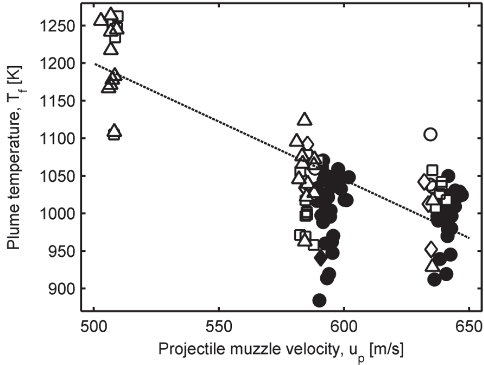
Figure 20. The number of plumes combusting is shown for each event as a function of estimated plume temperature and measured muzzle velocity of the projectile. Circles (○) indicate no flash; and diamonds (◇), squares (□), and triangles (△) represent 1, 2, and 3 plumes flashing. Configurations containing flash suppressant are shown with solid symbols and rarely flash. Three distinct groupings are observed corresponding to Full Charge, Charge 1, and Charge 2, from right to left.
